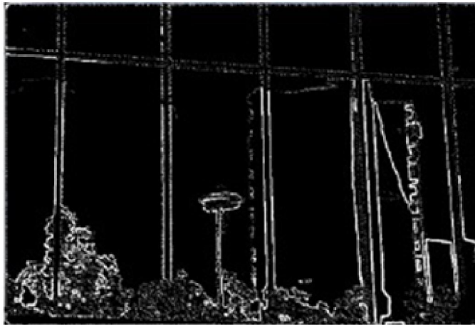
Canny
