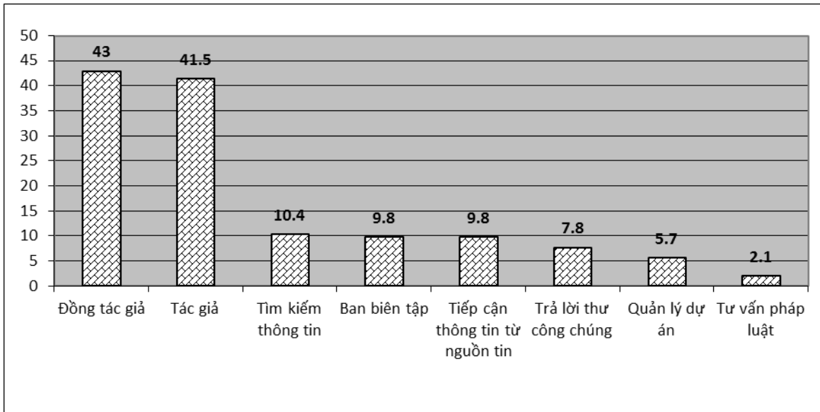
Descriptive Statistics
